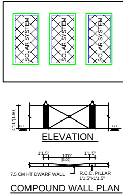
COMPOUND WALL PLAN
