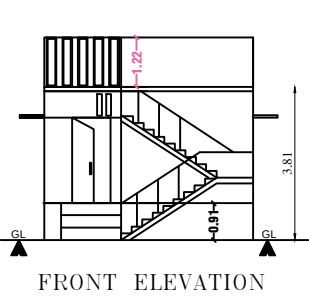
FRONT ELEVATION
