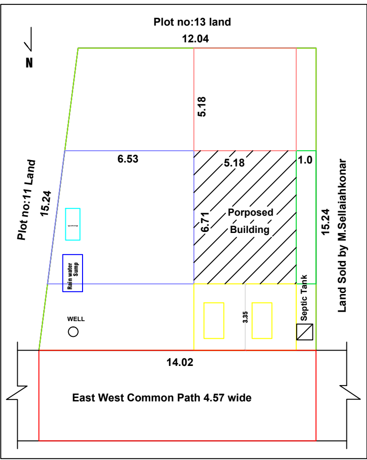
SITE PLAN CUM KEYPLAN
