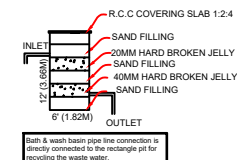
Detail of the Rain Water Harvesting System
