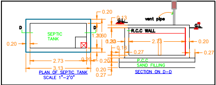
PLAN OF SEPTIC TANK SCALE 1"=2'0"
