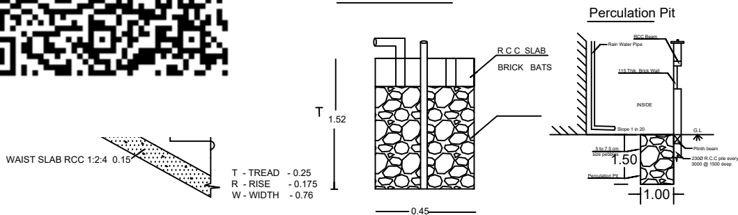
RAIN WATER STORAGE
