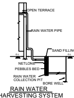
RAIN WATER HARVESTING SYSTEM
