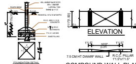
COMPOUND WALL PLAN
