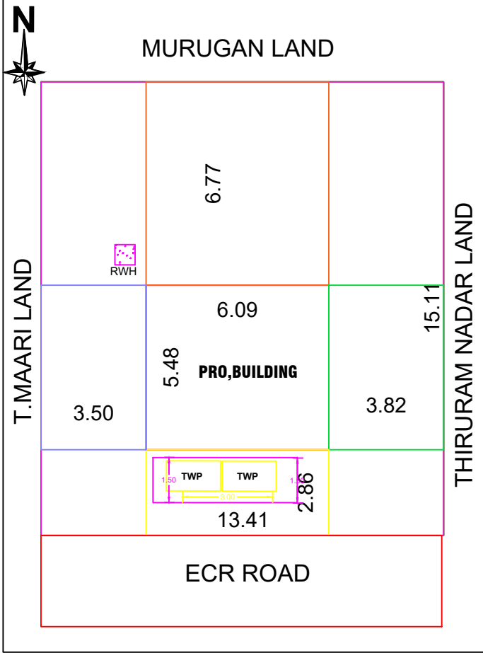
SITE PLAN
