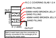
Detail of Rain Water Harvesting System
