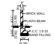
SECTION - CC
