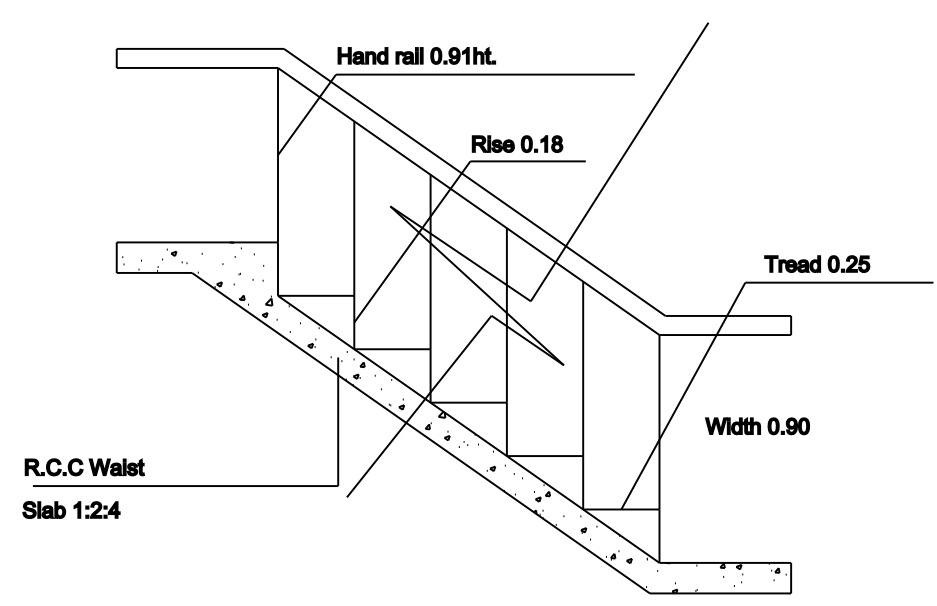
STAIRCASE DETAIL
