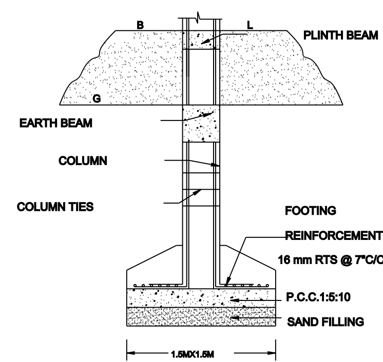
FOUNDATION DETAIL
