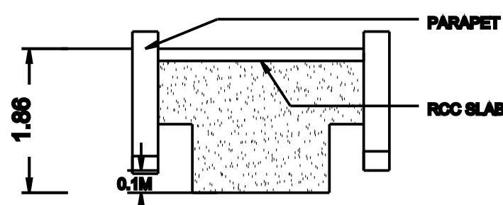
SECTION
