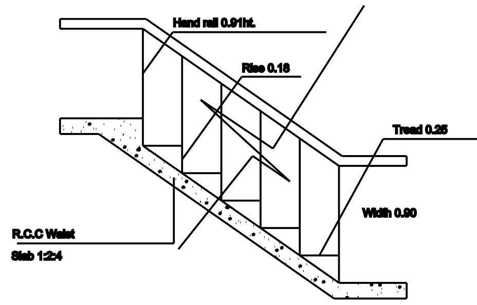
STAIRCASE DETAIL
