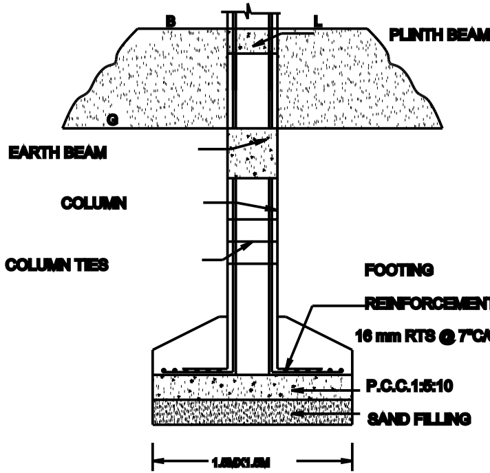
FOUNDATION DETAIL
