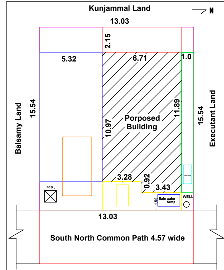
SITE PLAN CUM KEYPLAN
