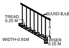
STAIRCASE DETAILS
