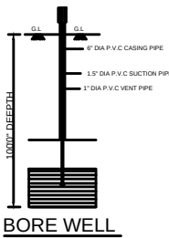
BORE WELL
