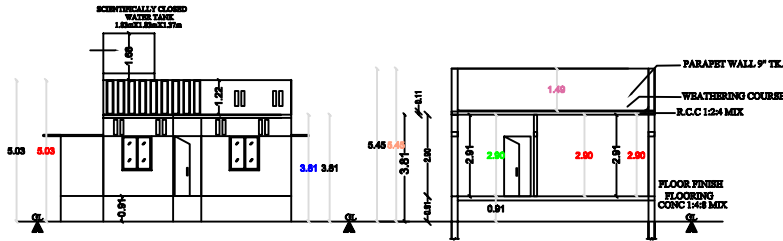
FRONT ELEVATION
