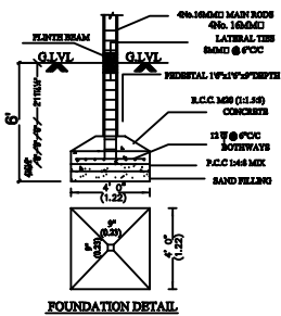
FOUNDATION DETAIL
