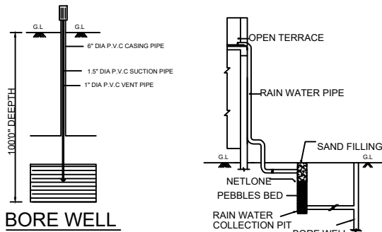
RAIN WATER HARVESTING SYSTEM
