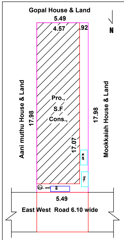
SITE PLAN & KEY PLAN (1:100)
