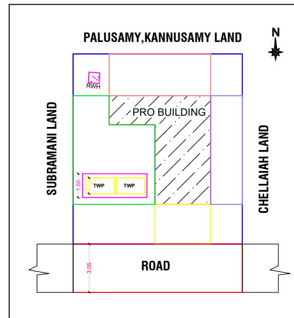
SITE PLAN
