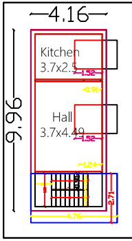
EAST WEST ROAD WIDTH 3.05M SITE PLAN & GROUND FLOOR PLAN
