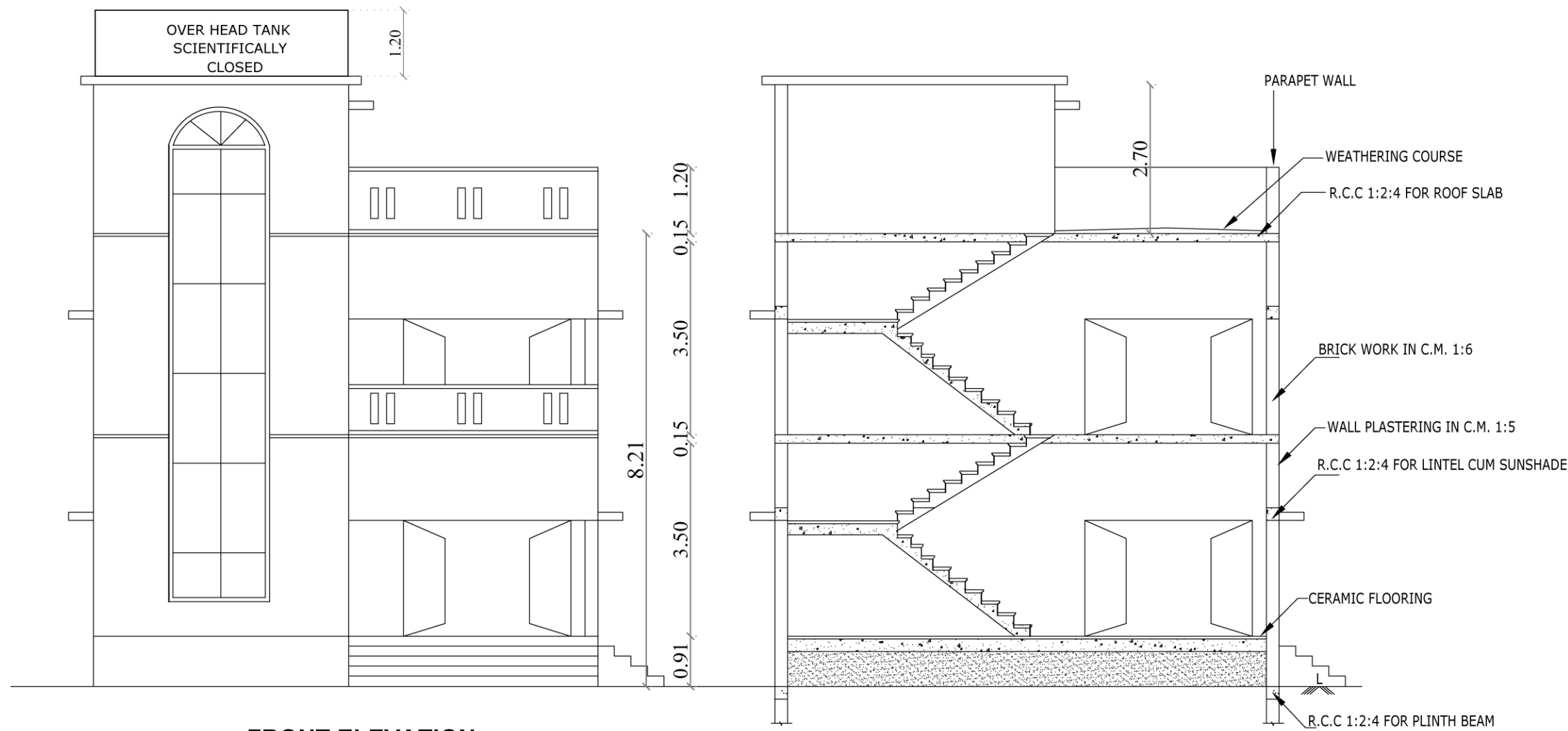
SECTION ON "AB" BLOCK No. 1
