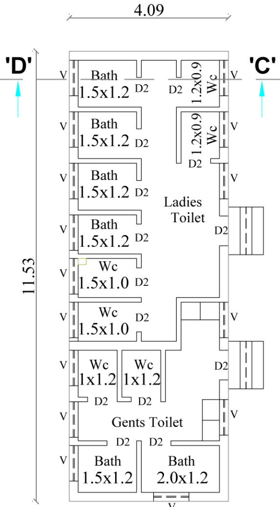
GROUND FLOOR PLAN BLOCK No. 2
