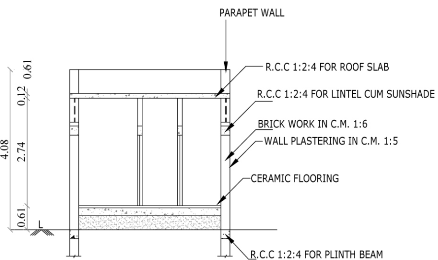
SECTION ON "CD" BLOCK No. 2
