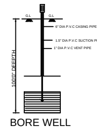
BORE WELL
