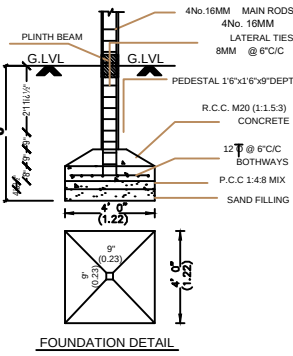
FOUNDATION DETAIL
