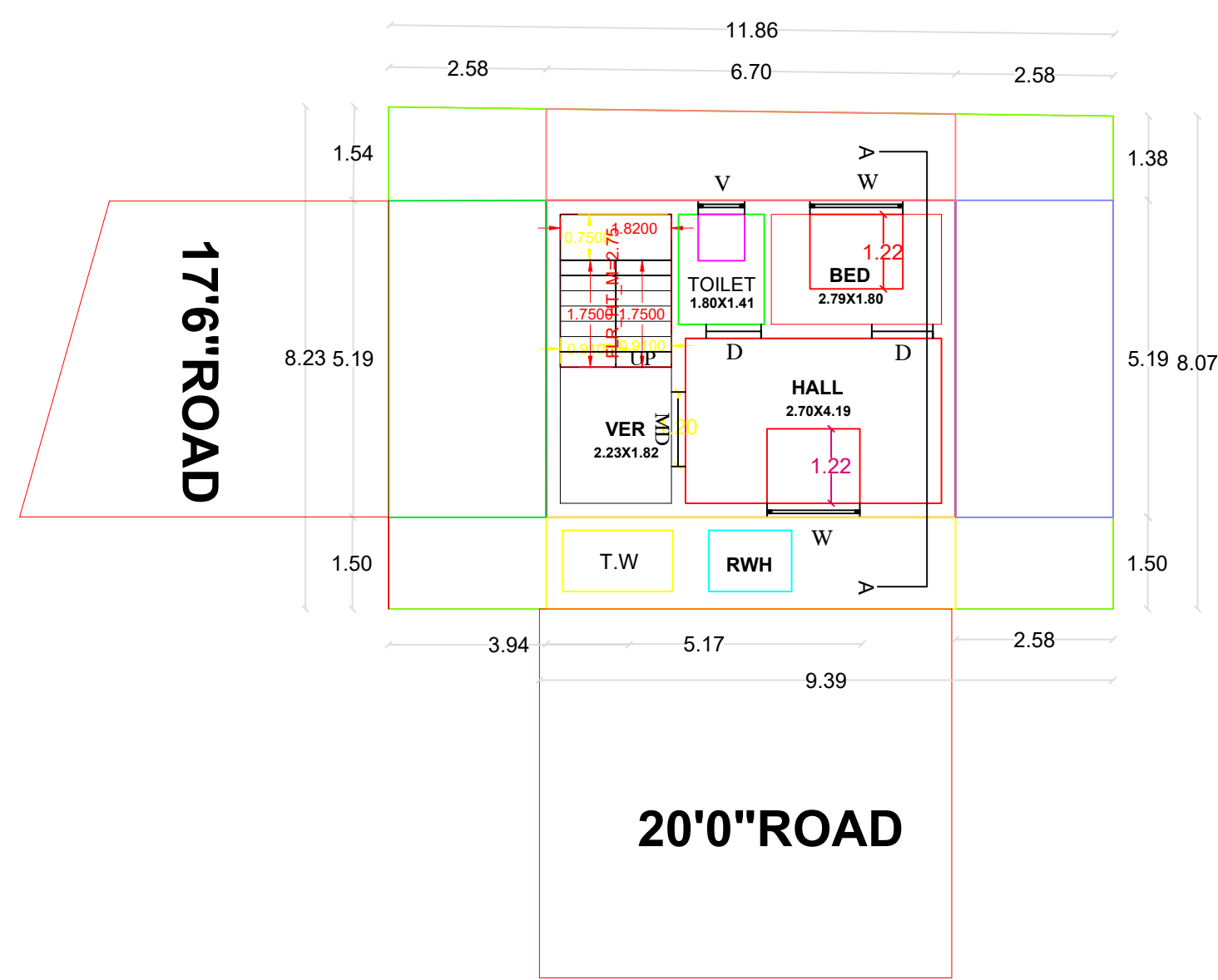
PLAN CUM GROUND FLOOR PLAN
