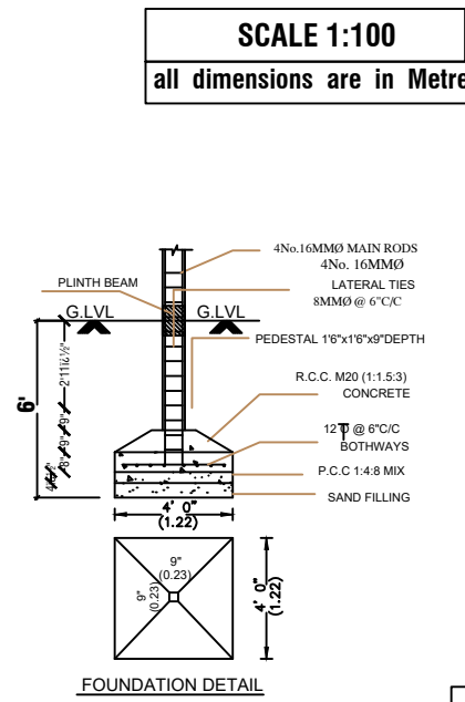
FOUNDATION DETAIL
