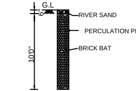
PERCOLATION PIT
