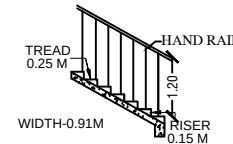
STAIRCASE DETAILS
