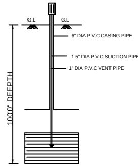
BORE WELL
