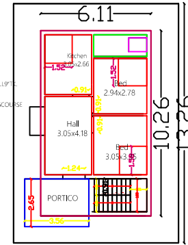
SITE PLAN CUM GROUND FLOOR PLAN
