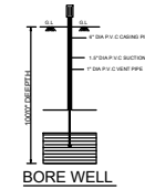
BORE WELL
