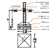
FOUNDATION DETAIL
