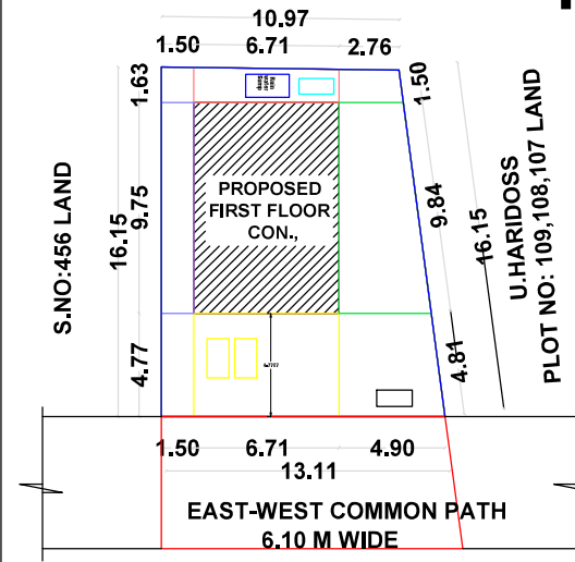
SITE PLAN & KEY PLAN (1:100)
