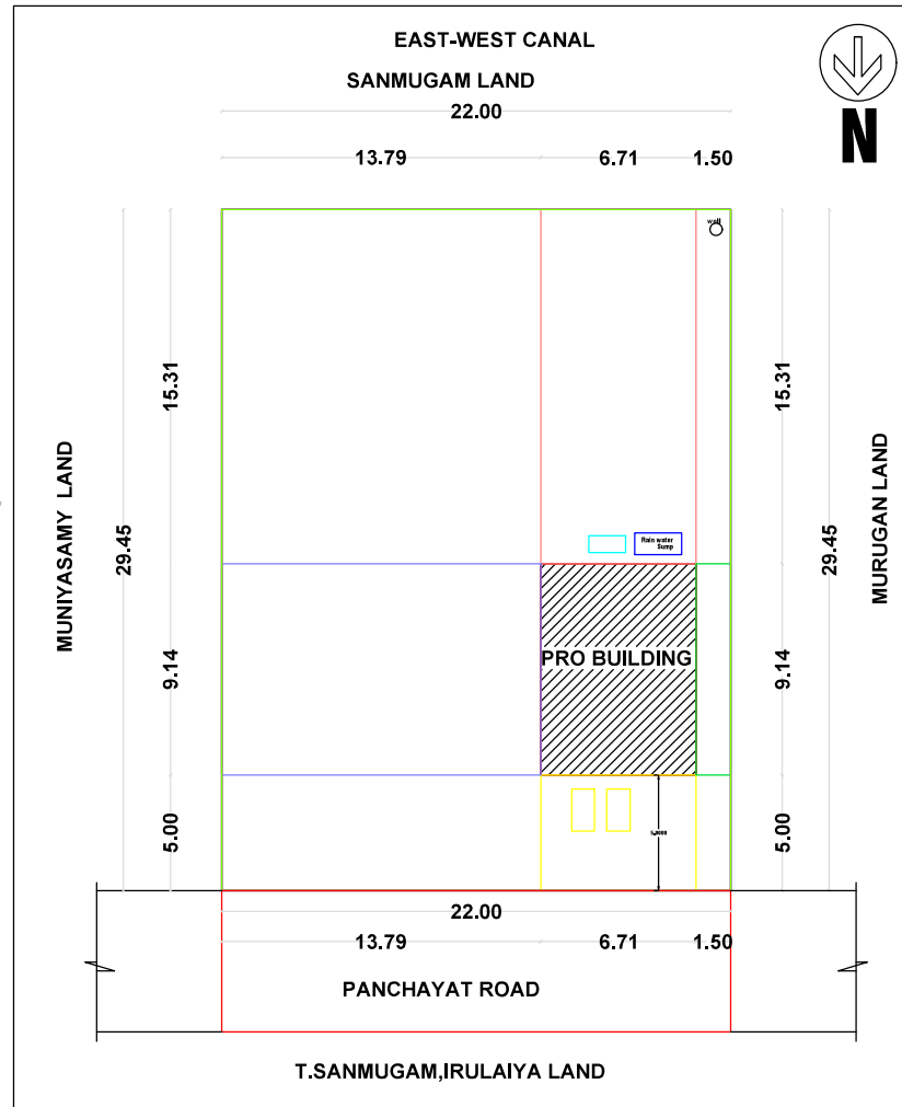
SITE PLAN & LOCATION
