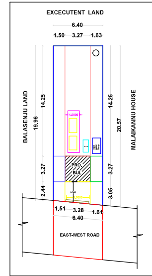
SITE PLAN & KEY PLAN
