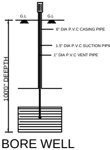
BORE WELL
