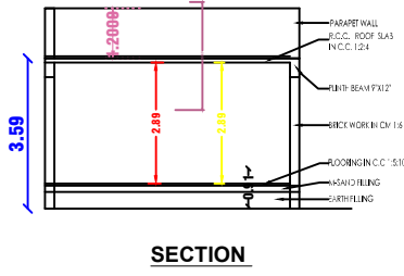
SECTION
