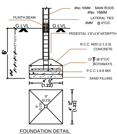
FOUNDATION DETAIL
