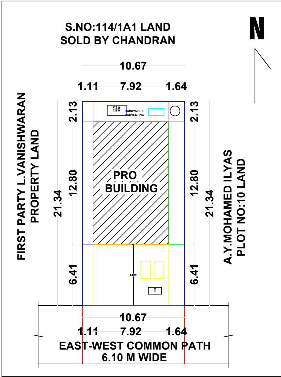
SITE PLAN & KEY PLAN (1:100)
