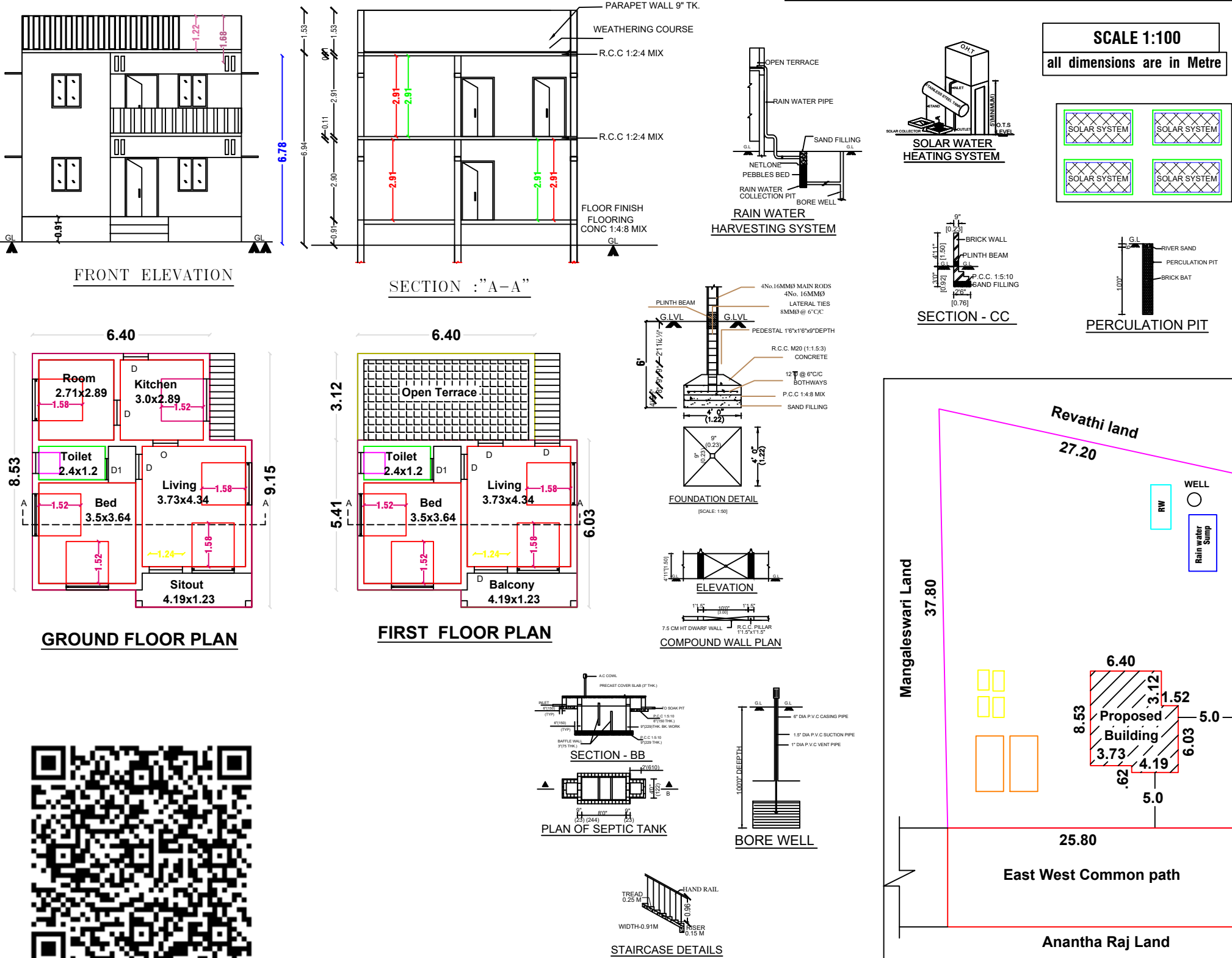
SITE PLAN CUM KEYPLAN
