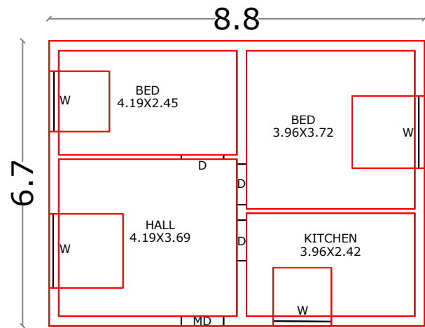
PROPOSED RESIDENTIAL GROUND FLOOR
