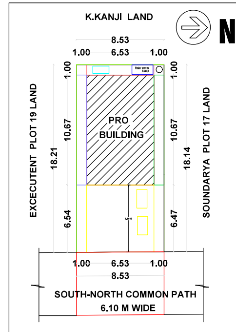
SITE PLAN & LOCATION
