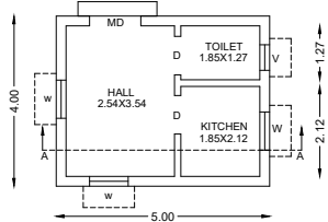
FLOOR PLAN
