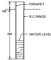
C.S. OF WELL
