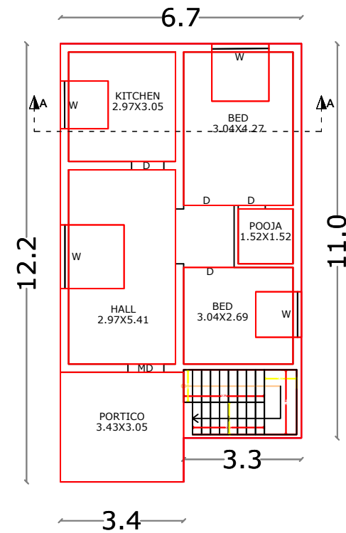
PROPOSED RESIDENTIAL GROUND FLOOR
