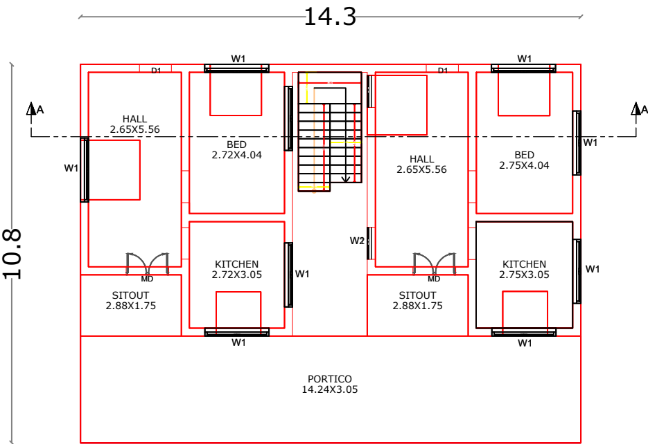
PROPOSED RESIDENTIAL GROUND FLOOR
