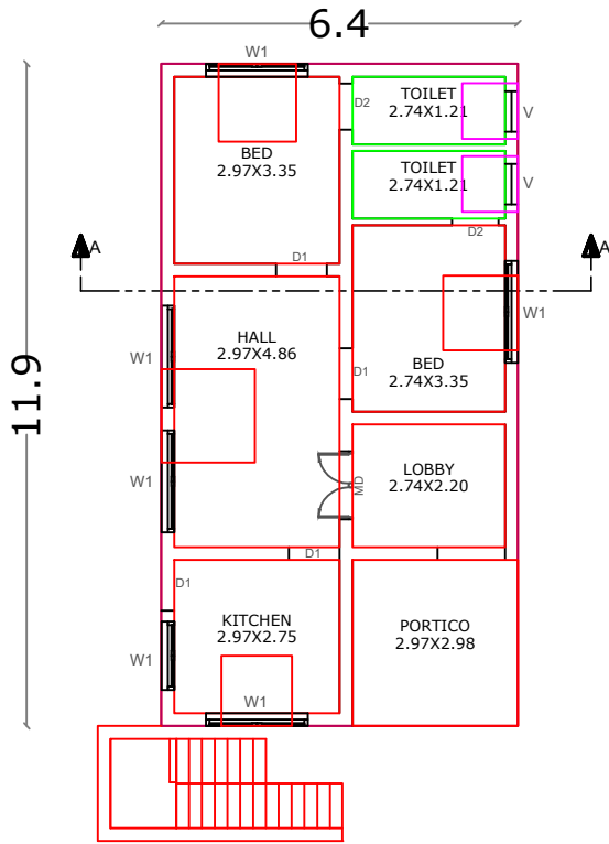
PROPOSED RESIDENTIAL GROUND FLOOR
