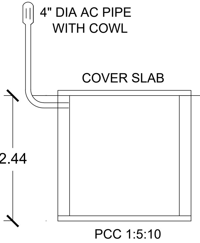
SEPTIC TANK
