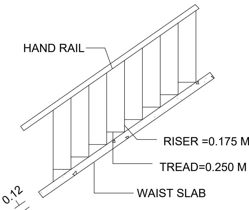
STAIRCASE DETAILS
