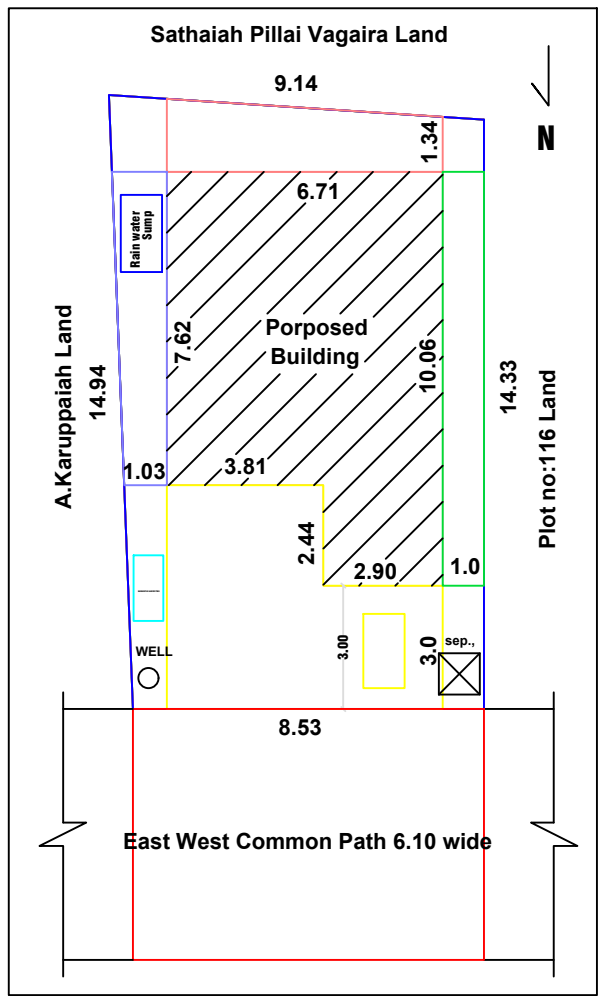
SITE PLAN CUM KEYPLAN
