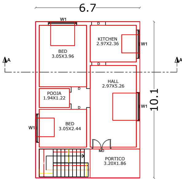
PROPOSED RESIDENTIAL GROUND FLOOR
