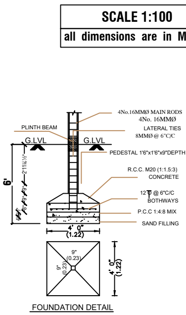
FOUNDATION DETAIL
