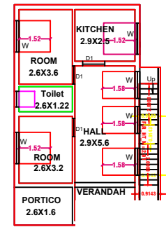
GROUND F
