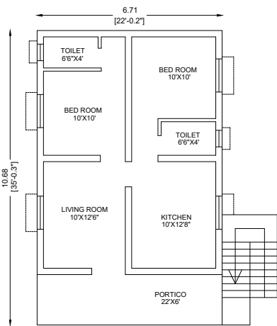
EXT.GROUND FLOOR PLAN
