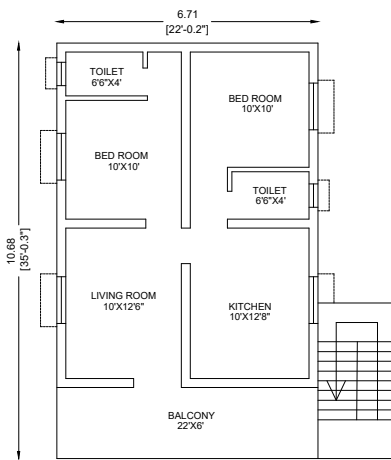
EXT.FIRST FLOOR PLAN
