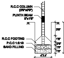
FOUNDATION DETAILS (SCALE 1\"/>
