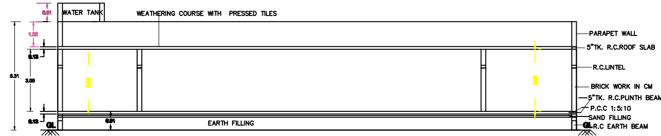
SECTION AA
