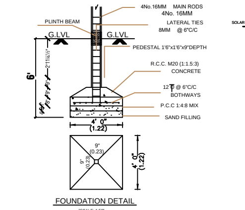
FOUNDATION DETAIL (SCALE: 1:50)
