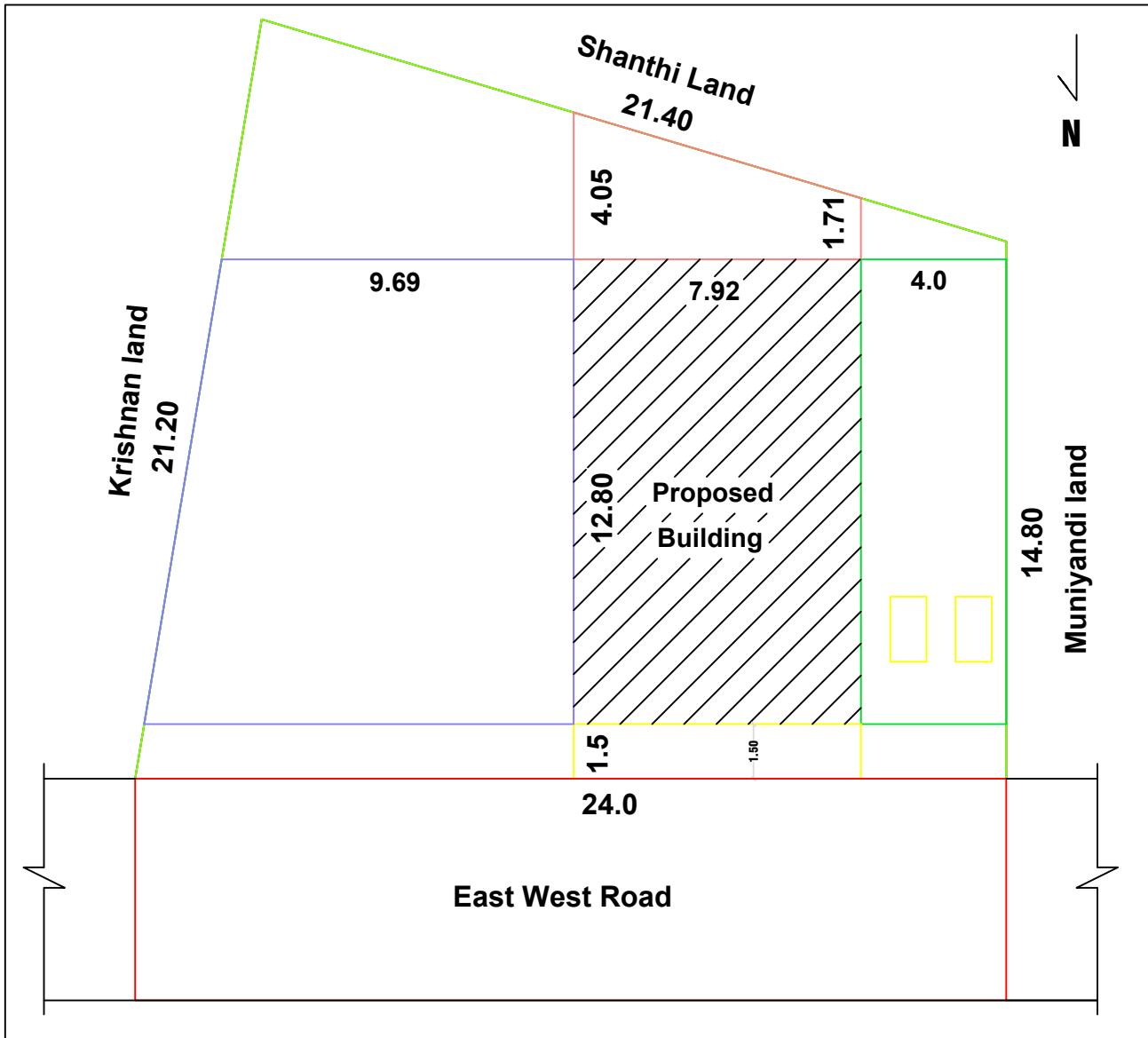
SITE PLAN CUM KEYPLAN
