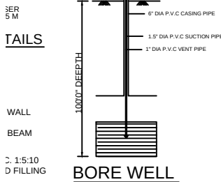
BORE WELL
