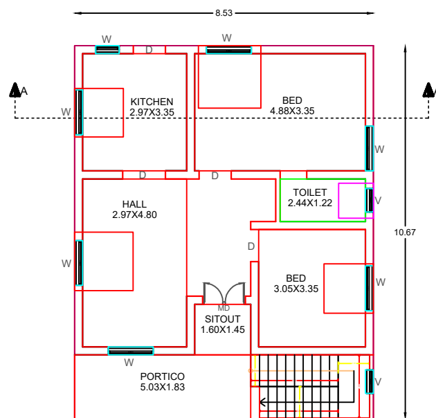
PROPOSED RESIDENTIAL GROUND FLOOR
