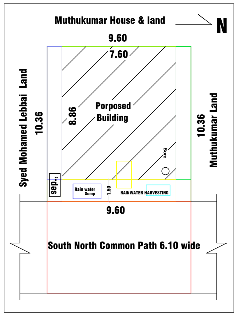
SITE PLAN CUM KEYPLAN
