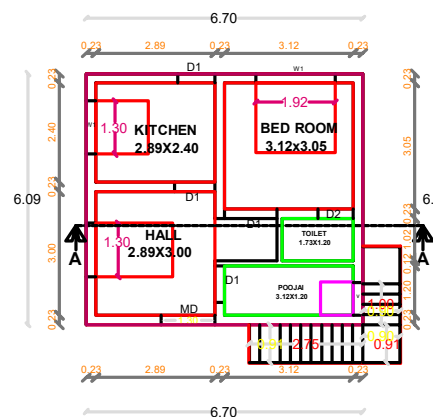
GROUND FLOOR PLAN PROPOSED
