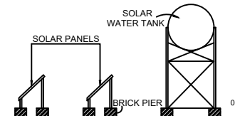
SECTION OF SOLAR HEATER
