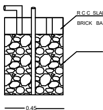
RAIN WATER STORAGE
