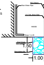
Percolation Pit
