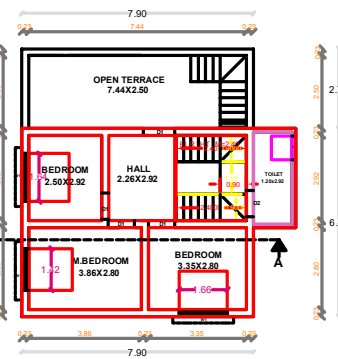
FIRST FLOOR PLAN PROPOSED
