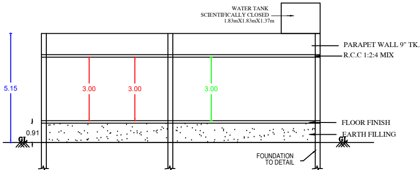
SECTION AB
