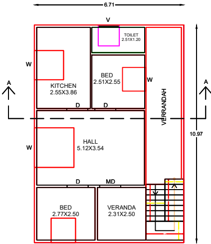
EXISTING RESIDENTIAL GROUND FLOOR
