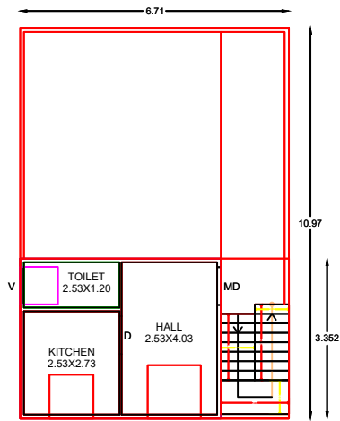
PROPOSED RESIDENTIAL SECOND FLOOR
