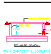
RWH_CAPACITY_L=2000LTRS
