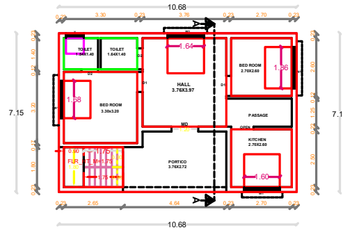
GROUND FLOOR PLAN PROPOSED
