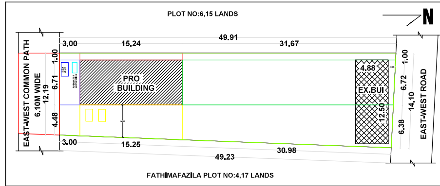
SITE PLAN & KEY PLAN (1:100)
