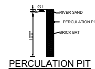
PERCOLATION PIT
