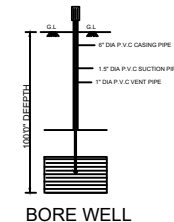
BORE WELL
